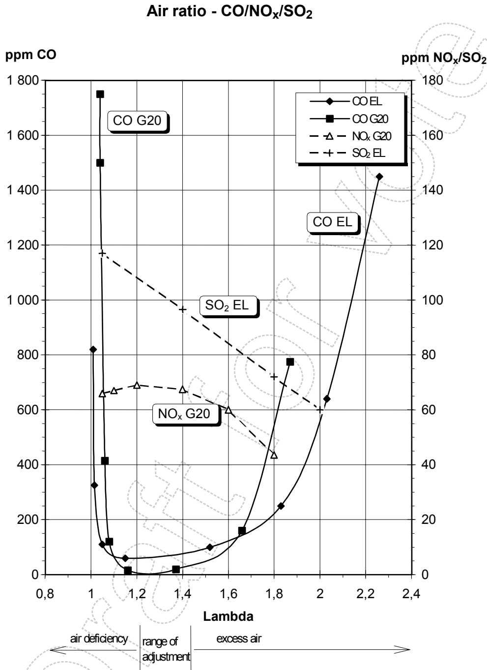
Figure B.1 – CO, NO and SO 2 variation with air ratio
